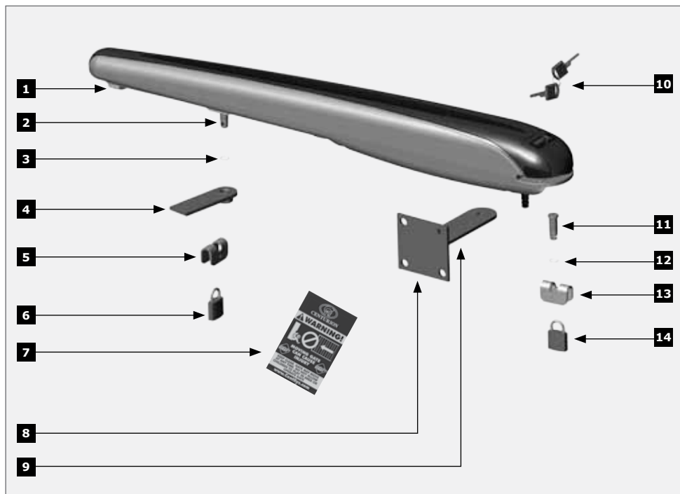
FIGURE 4. VECTOR2 SWING GATE MOTOR
