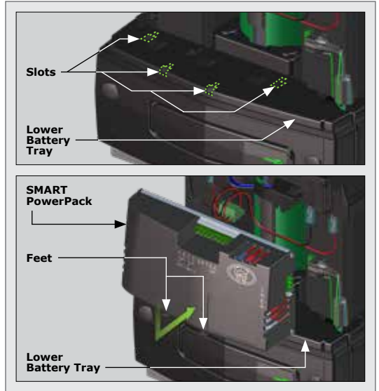
FIGURE 8. SMART POWERPACK PLACEMENT
