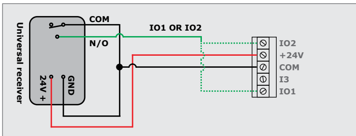
FIGURE 85. WIRING A UNIVERSAL RECEIVER TO THE SDO5 SMART+
