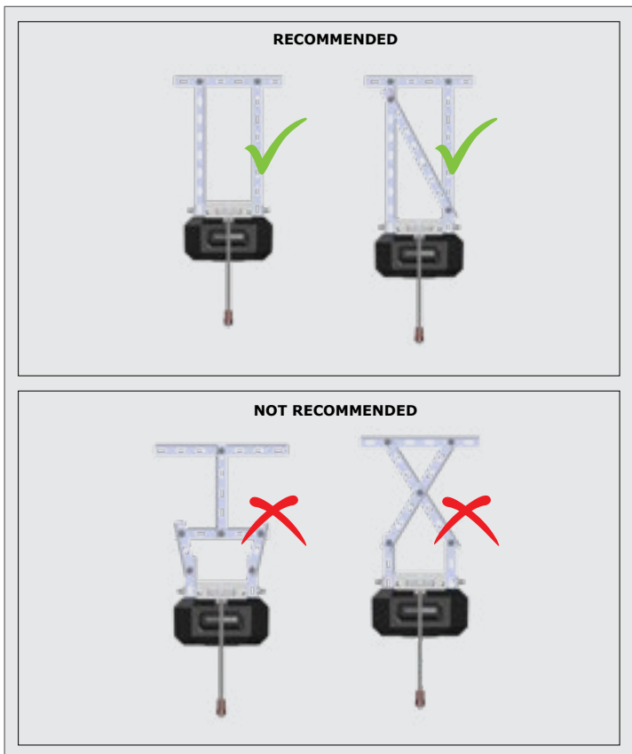
FIGURE 32. CORRECT AND INCORRECT MOUNTING CONFIGURATIONS
