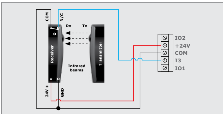
FIGURE 83. WIRING PHOTON SAFETY BEAMS TO THE SDO5 SMART+ (FOUR-WIRE)
