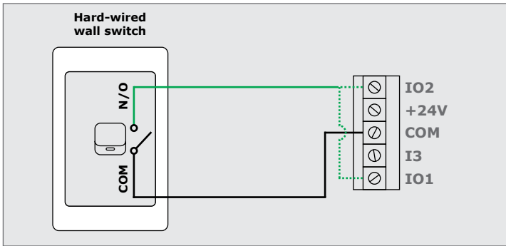
FIGURE 86. HARD-WIRING A WALL SWITCH TO THE SDO5 SMART+
