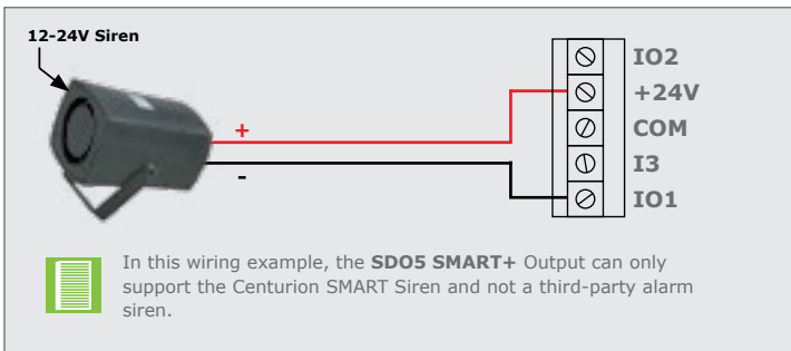
FIGURE 87. SMART SIREN CONNECTED TO SDO5 SMART+
