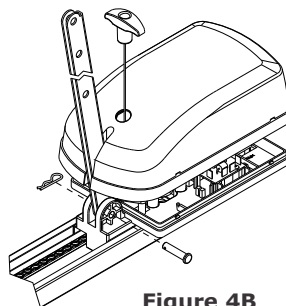
FIGURE 4. ATTACHING STRAIGHT TOWING ARM
